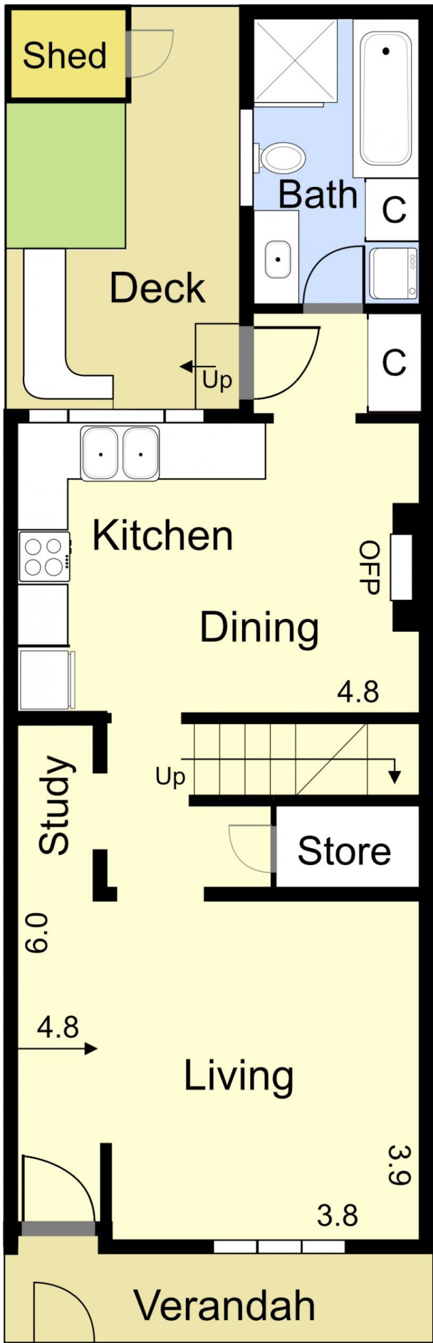
Ground Floor
